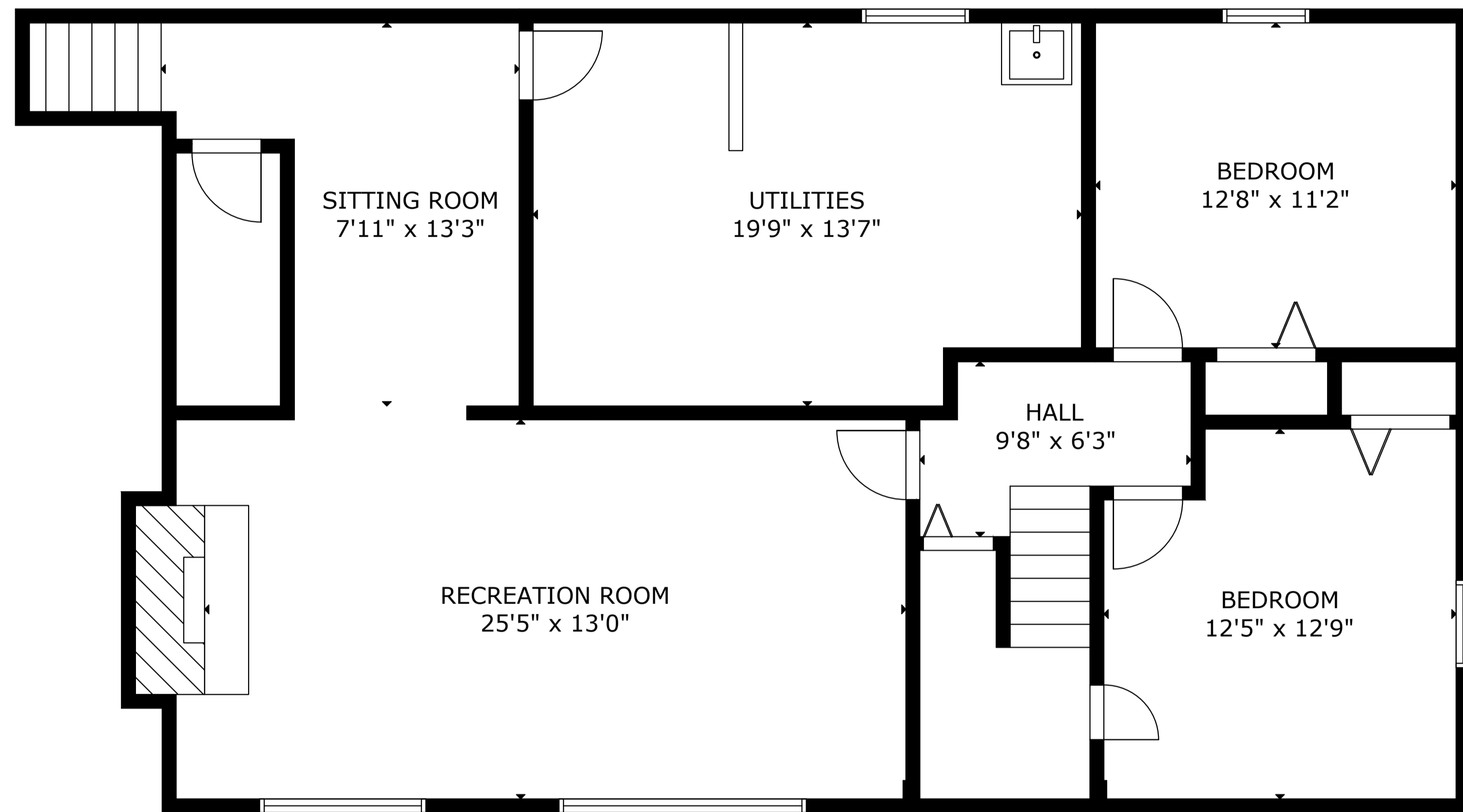
FLOOR 1
