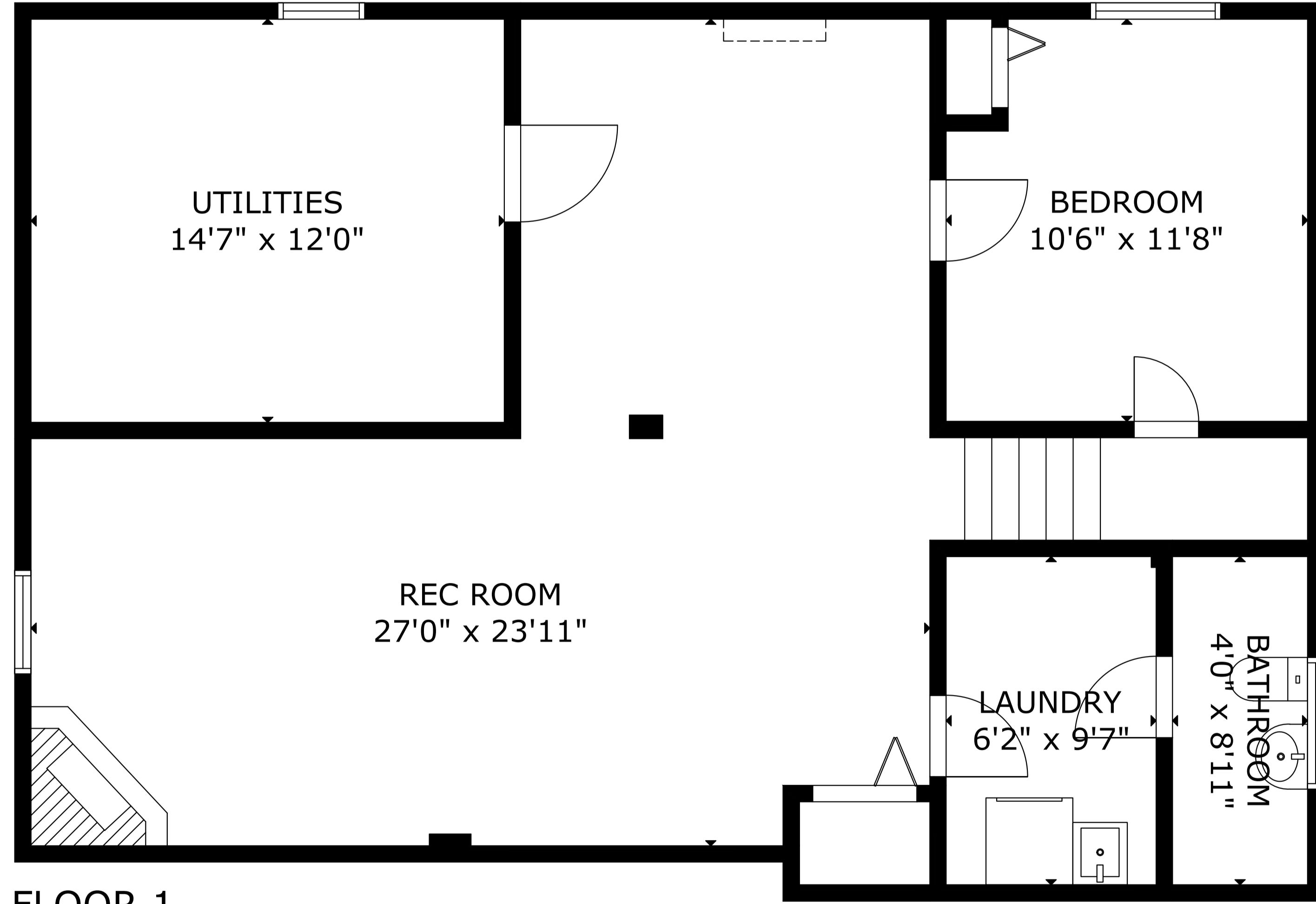
FLOOR 1
